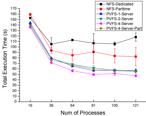
Figure 3: BTIO total execution time
