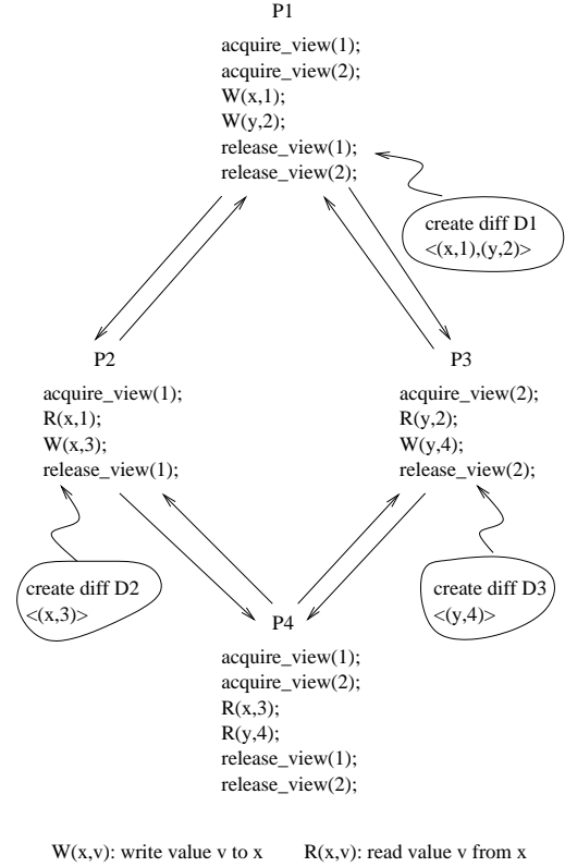
Figure 1: A failure scenario for diff integration in ScC programs) or acquire_lock and release_lock (as in TreadMarks) respectively, diff integration will result in the same incorrect memory consistency. Therefore, ScC and TreadMarks cannot adopt the VOUPID protocol to improve the performance of DSM systems.
